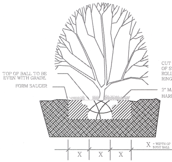
BALLED & BURLAPPED
